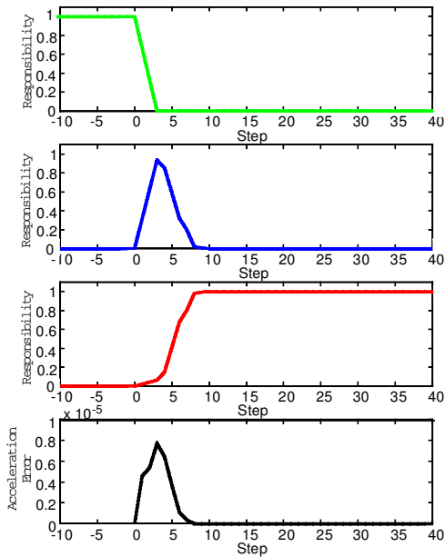
Figure 5: Responsibility predictions based on contextual information of two-dimensional object shapes (top three traces) and corresponding acceleration error of control induced by an unusual shape-dynamic pairing (bottom trace).
